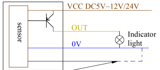
PNP signal output: wiring method to connect to controller or MCU
