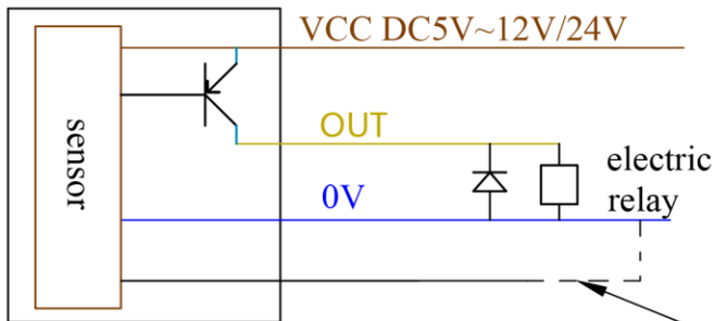
Normally open/normally closed output selection
